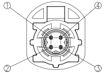
PINNING
