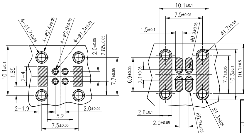
PCB LAYOUT
